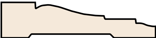
COLONIAL CASING #36I 11/16" x 2-3/4"
