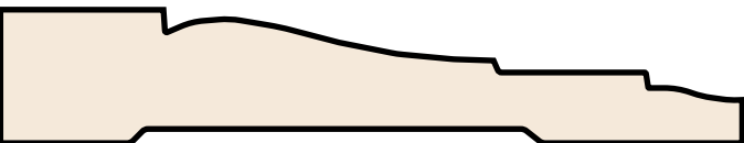
COLONIAL CASING #36I 11/16" x 3-1/2"
