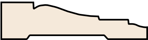
COLONIAL CASING #36I 11/16" x 2-1/2"
