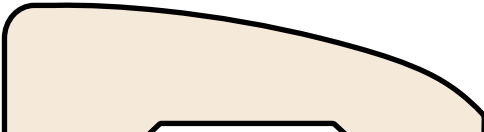
RANCH CASING #315 11/16" x 2-1/2"
